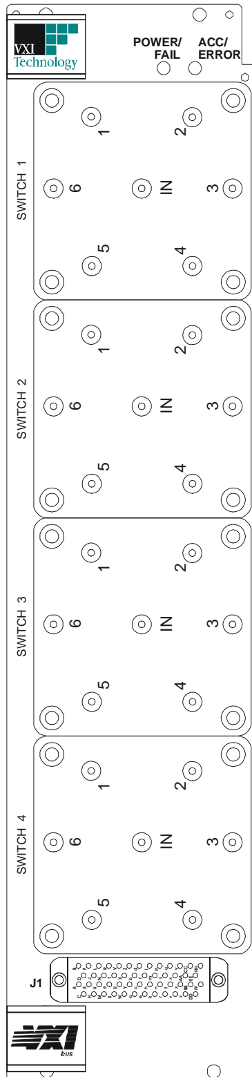
FIGURE 4-12 SM7001L FRONT PANEL
