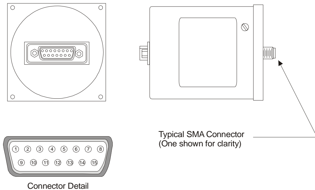
FIGURE 4-13 SWITCH OPTION (SM7374L) TO SM7001L CONNECTION
