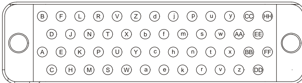
FIGURE 4-26 50-PIN CONNECTOR DETAIL
