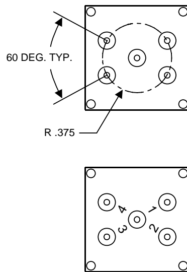
FIGURE 4-5 SM7272 - SP4T
